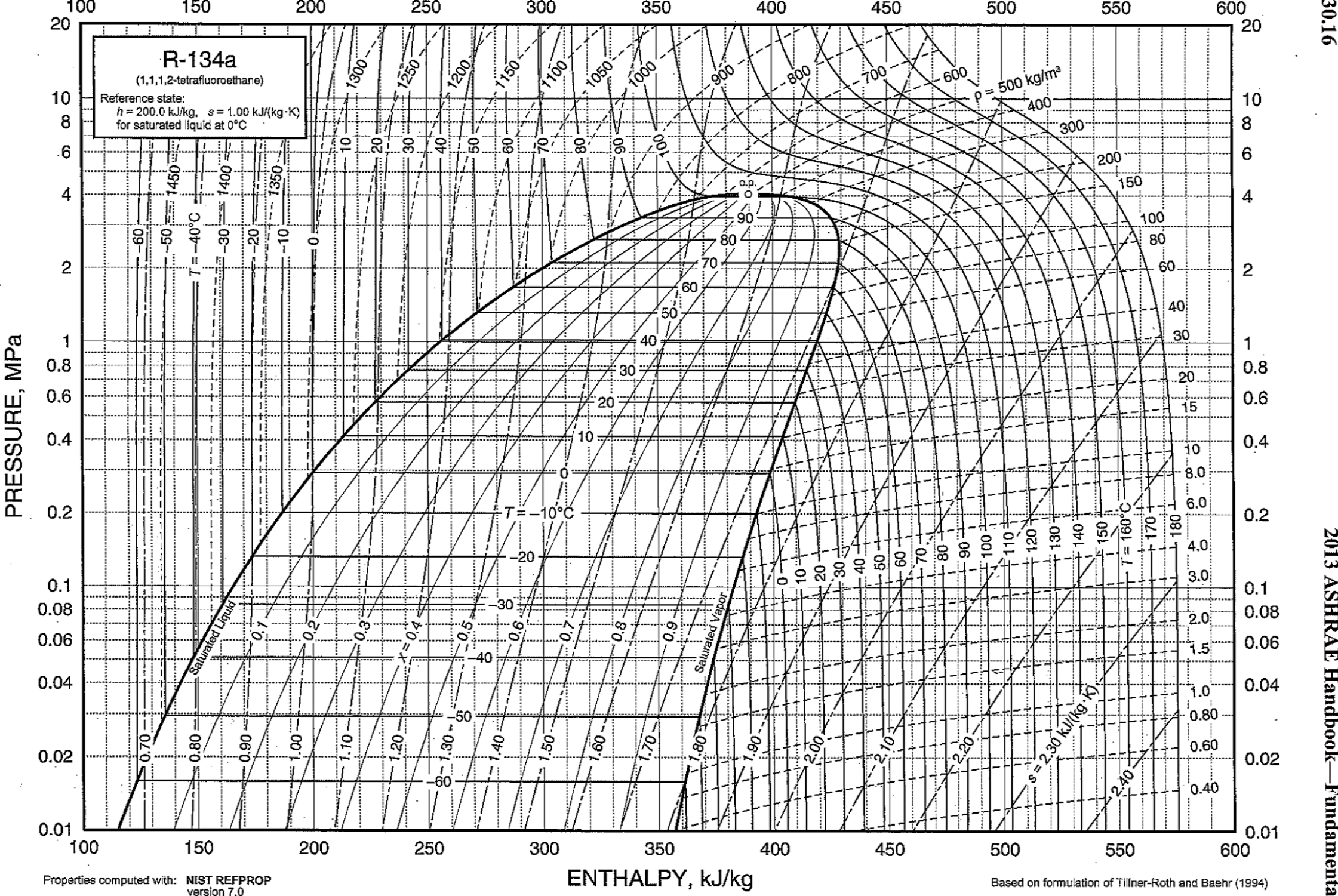
Fig. 8 Pressure-Enthalpy Diagram for Refrigerant 134a
