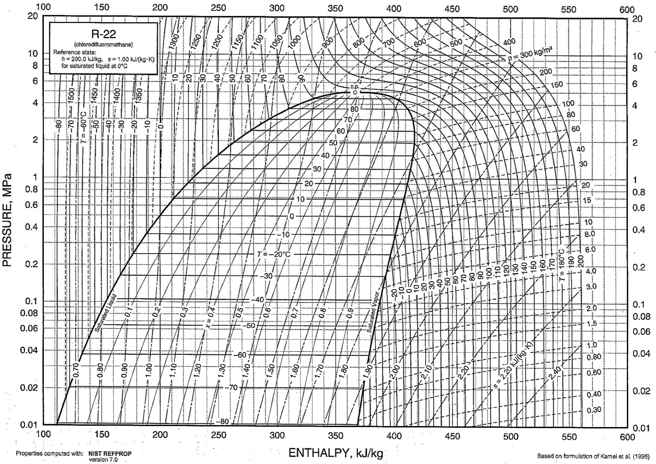
Fig. 2 Pressure-Enthalpy Diagram for Refrigerant 22
