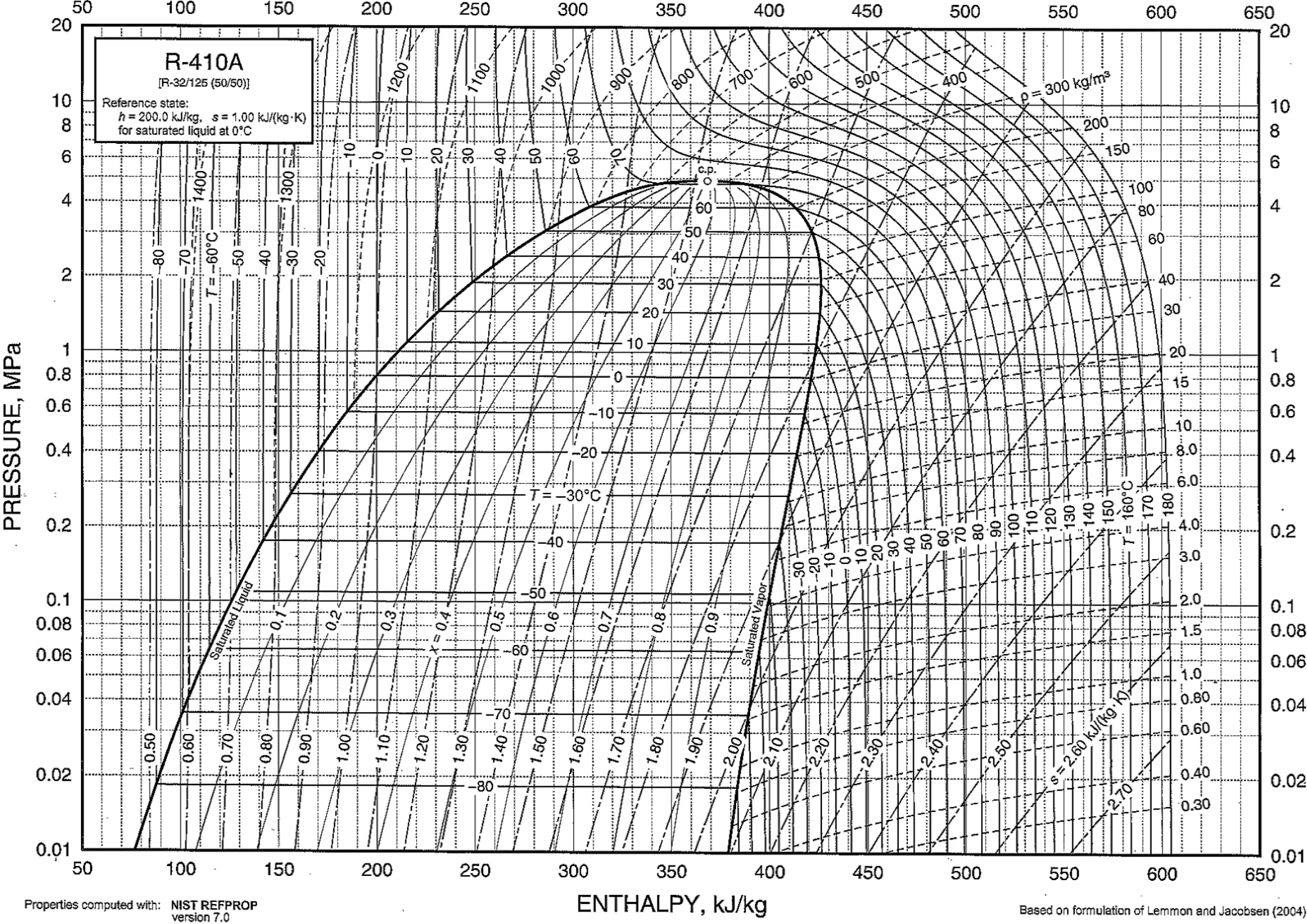
Fig. 16 Pressure-Enthalpy Diagram for Refrigerant 410A
